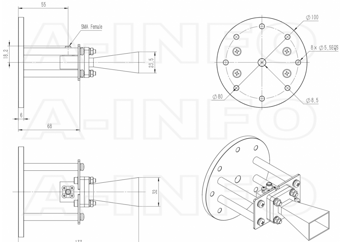
SMA-Female Output with Round Mounting Bracket (Option, P/N: LB-62-10-C-MB)
