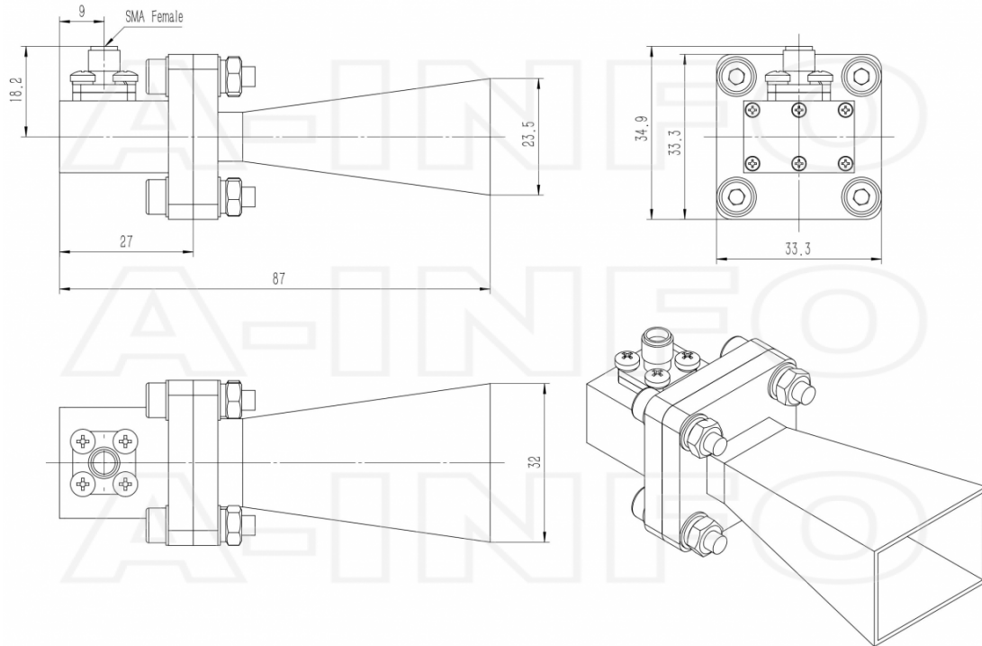
SMA-Female Output (P/N: LB-62-10-C-SF)
