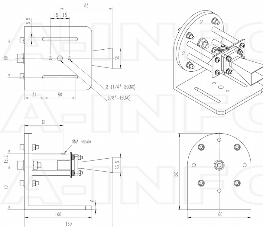
SMA-Female Output with L Type Mounting Bracket (Option, P/N: LB-62-10-C-MBL)
